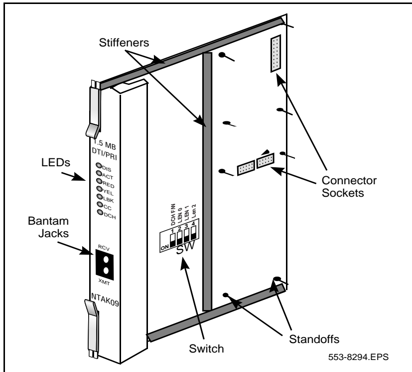
Figure 2 NTAK09 DTI/PRI circuit card
