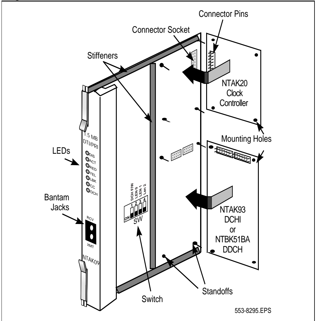
Figure 4 Daughterboard installation
