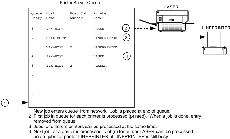
Figure 4. Print Job Processing
